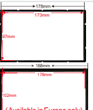
Installation Frame
